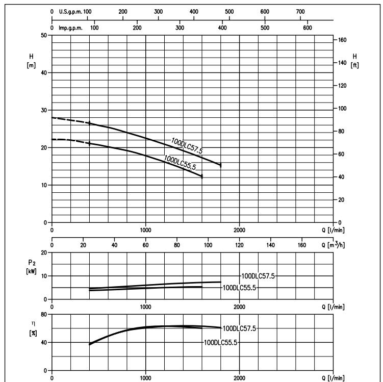
100DLC55.5 (5.5 kW) PERFORMANCE CURVES 100DLC57.5 (7.5 kW)
