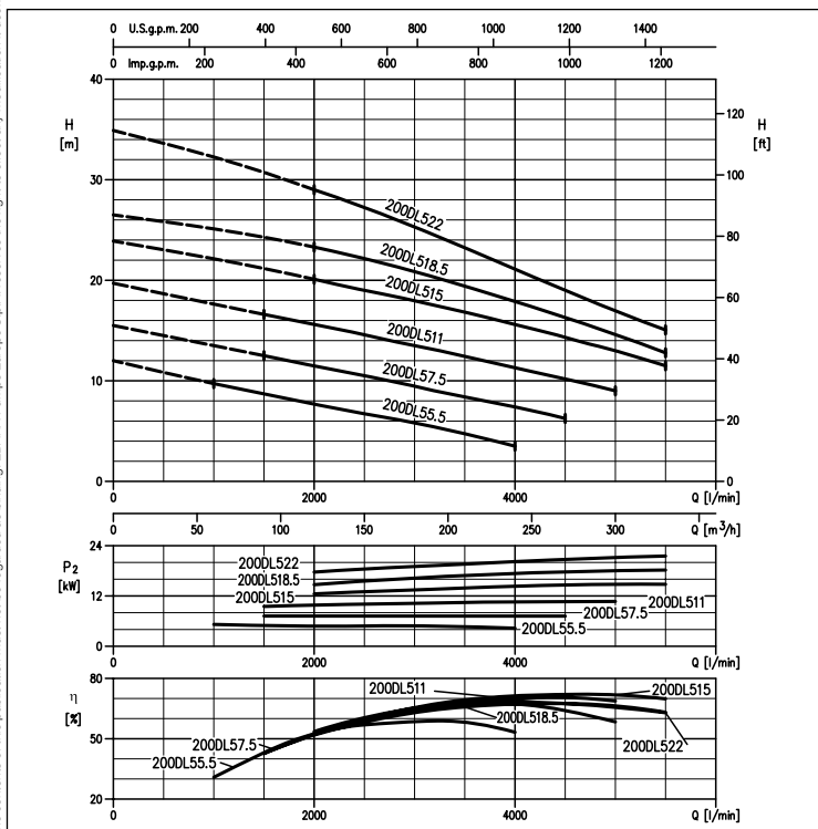
PERFORMANCE CURVES 200DL55.5 (5.5 kW) 200DL57.5 (7.5 kW) 200DL511 (11 kW) 200DL515 (15 kW) 200DL518.5 (18.5 kW) 200DL522 (22 kW)
