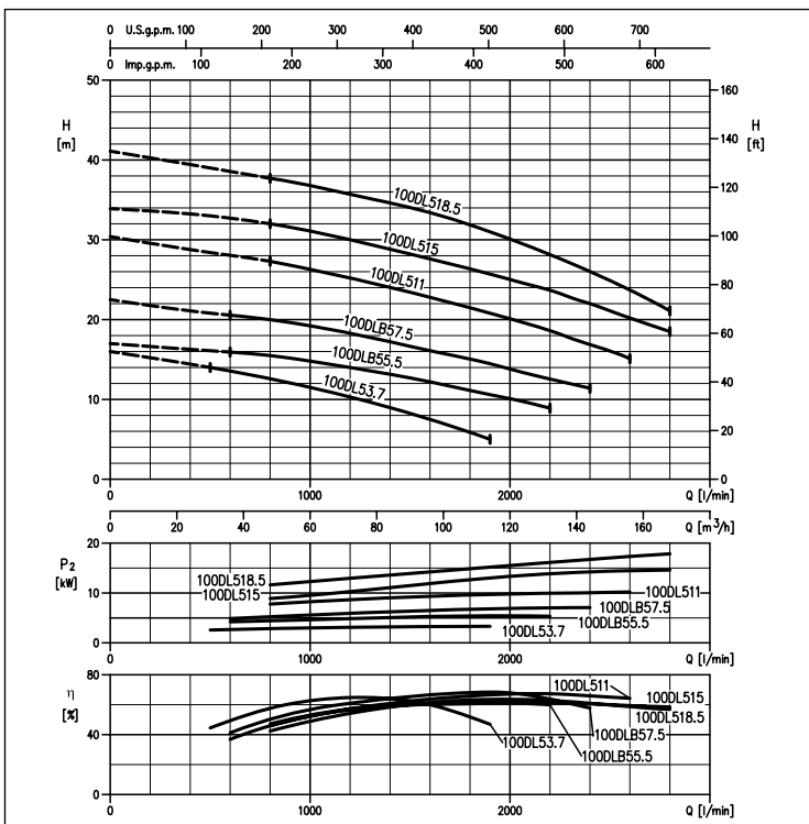
100DL53.7 (3.7 kW) 100DLB57.5 (7.5 kW) 100DL515 (15 kW)
