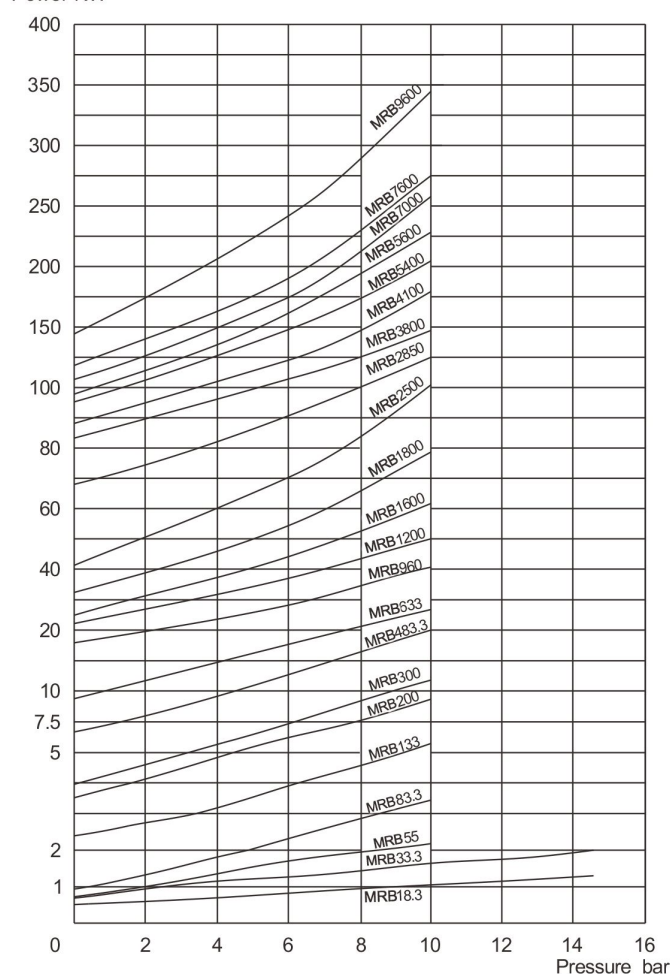
Power KW
